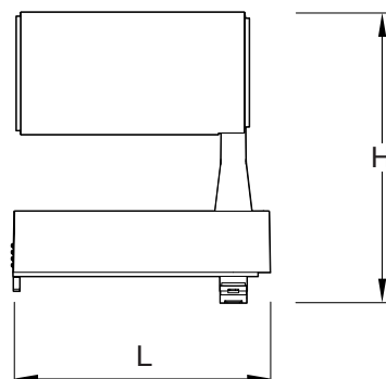
15W, Track
