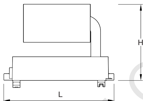
25W, Track
