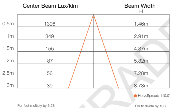
Illuminance at a distance
