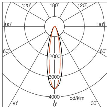
RGBW, 20° x 30°
