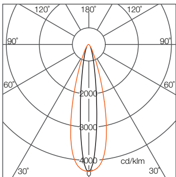
White, 15° x 30°
