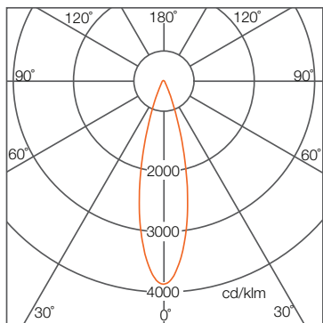
White, 25°
