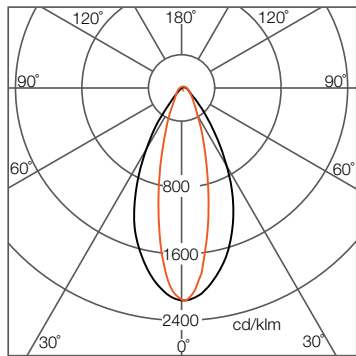
RGBW, 25° x 50°
