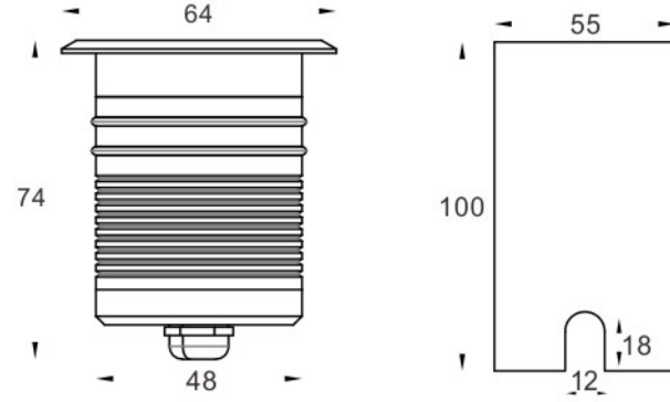
Physical Dimension(MM)
