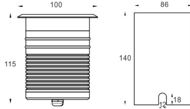
Physical Dimension(MM)
