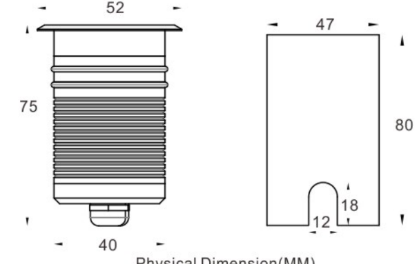
Physical Dimension(MM)
