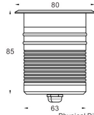
Physical Dimension(MM)
